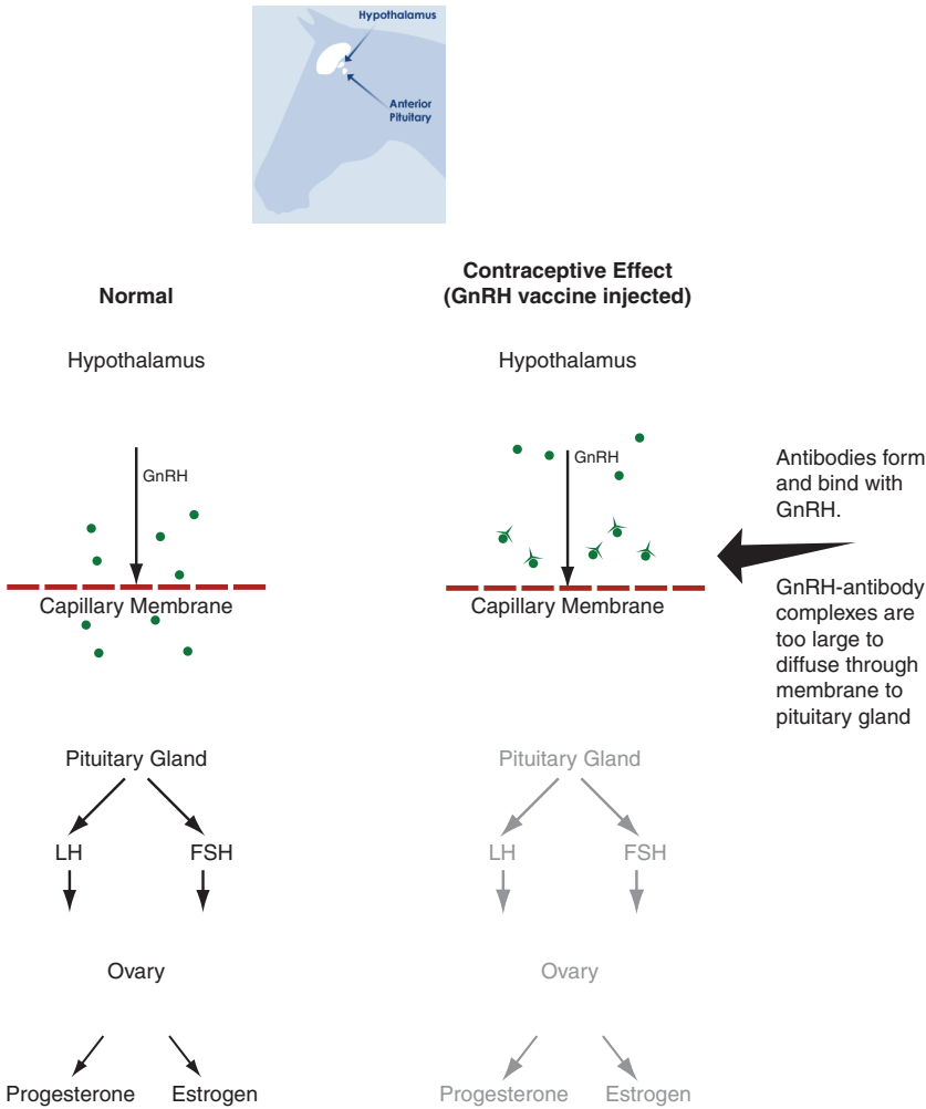
FIGURE 4-3 Mode of action of gonadotropin-releasing hormone (GnRH) vaccines. NOTE: Without GnRH to stimulate follicle-stimulating hormone (FSH) and luteinizing hormone (LH), there is no production of ovarian estrogen or progesterone and no ovulation. SOURCE: Adapted from Asa et al. (1996).
