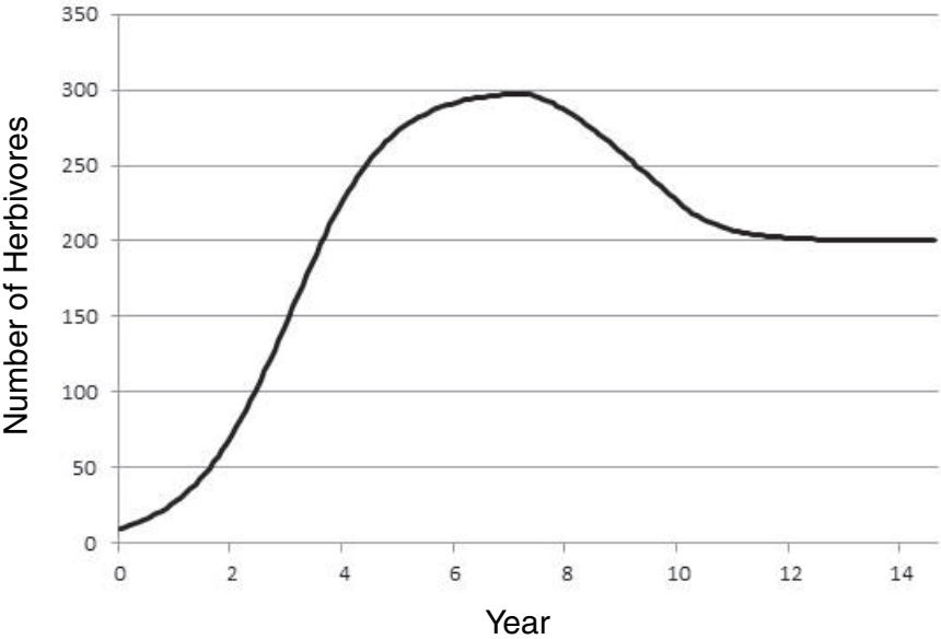
FIGURE 3-4 Large-herbivore population trajectory after an introduction. Herbivory causes a decline in plant production and thus in K . Here, K in the underlying logistic model declines linearly from 300 to 200 individuals from year 7 to year 10, and this results in a decline in herbivore population size.
