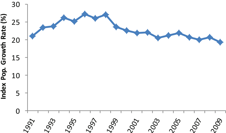
FIGURE 2-3 An index of population growth rate of free-ranging horses based on data on ages of 167,927 horses captured and removed from western rangelands in the United States to manage their abundance.
